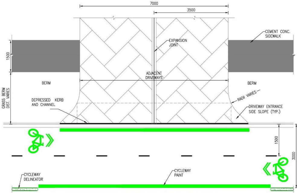
TYPICAL DUAL DRIVEWAY ACCESS OVER CYCLE LANE
