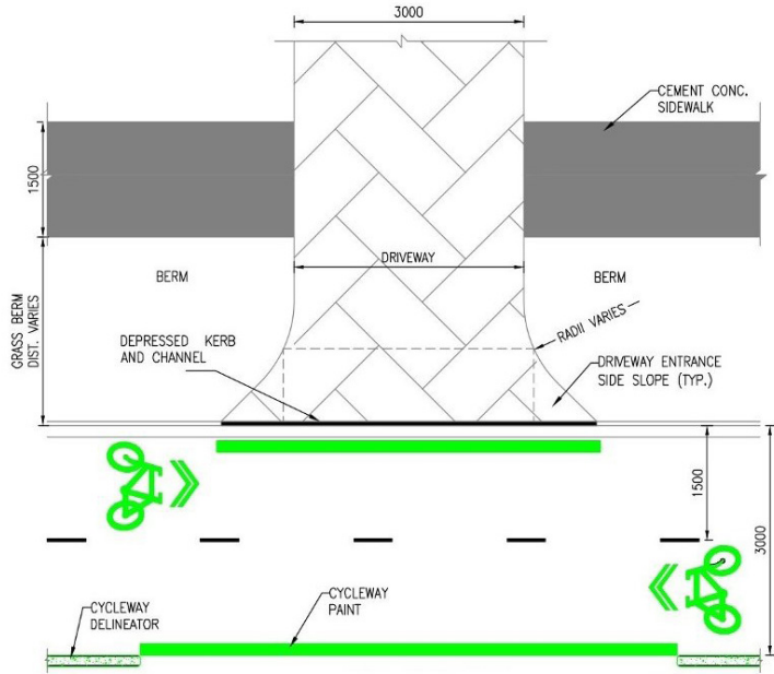
TYPICAL SINGLE DRIVEWAY ACCESS OVER CYCLE LANE
